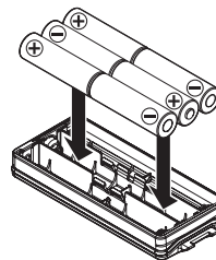
SBT-12 Alkaline Battery Tray
