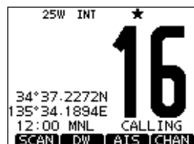
Transceiver's display
